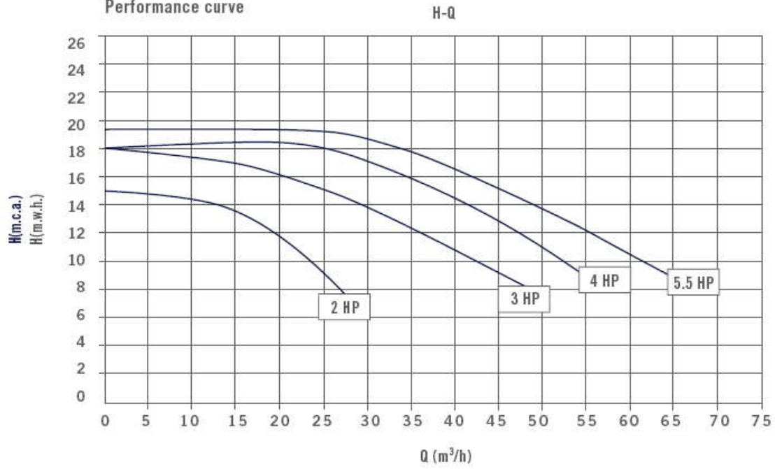
Courbe de rendement Performance curve
